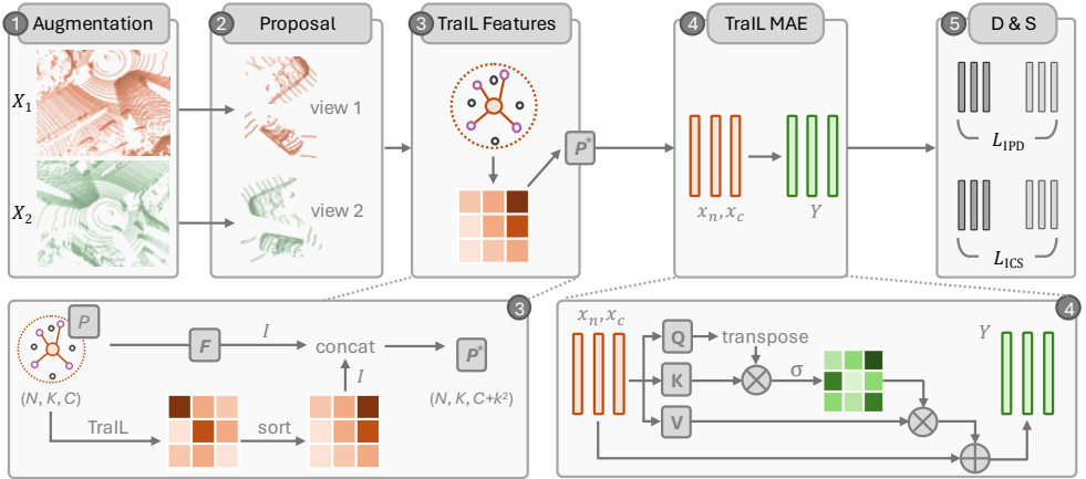
Figure 1: Our proposed TraIL architecture for 3D object detection leverages TraIL features from the point cloud. ❶ We take point cloud inputs as input and augment them with differing views. ❷ The augmented point clouds are sampled to the initial paired region proposals. ❸ The encoding module (TraIL MAE) extracts expressive proposal representations by considering the geometric relations among points within each proposal. ❹ We extract the concatenated features with the Multi-Head Attention Encoding Module (TraIL MAE). ❺ Inter-Proposal Discrimination (IPD) and Inter-Cluster Separation (ICS), i.e. D&S module [6] are subsequently enforced to optimize the whole network.
