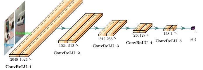
Fig. 5. Network architecture of the contrastive regression module.
